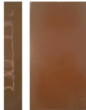
Si 57® E with and without cut AFTER testing
